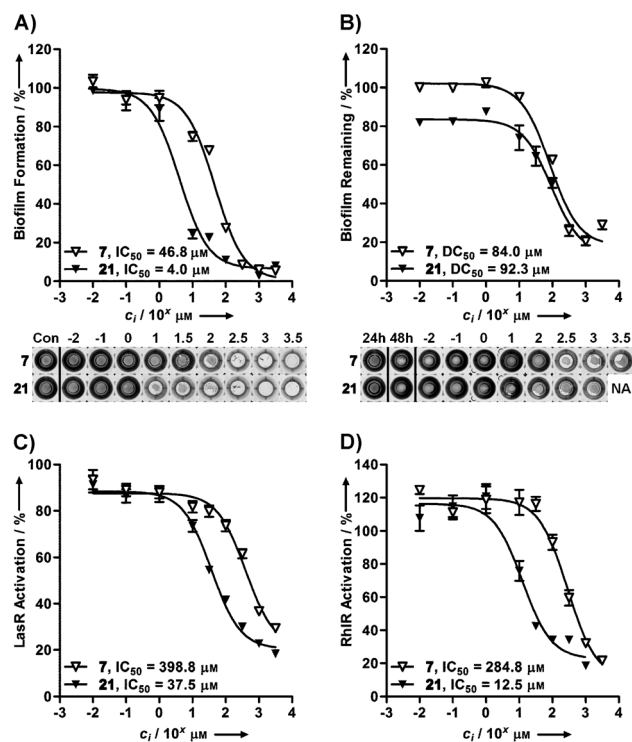
Figure 2. Dose-response curves and images of crystal violet biofilm inhibitory (A), and dispersion (B) assays for 7 and 21 in P. aeruginosa (PAO1). NA = not available. Dose-response curves for 7 and 21 in P. aeruginosa PAO1/ plasi -LVAgfp (C), and PAO1/ pRhI -LVAgfp (D) QS reporter strains.
