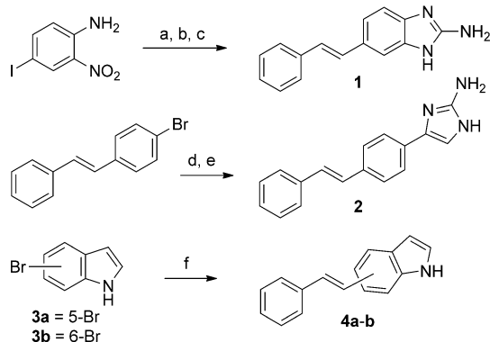
Scheme 1. Reaction conditions for the synthesis of stilbene derivatives: a) styrene, Pd(OAc) 2 , CH 3 CN, DIPEA, 80 °C, 76 %; b) SnCl 2 ·2 H 2 O, EtOAc, 80 °C; c) CNBr, MeOH/H 2 O (1:1), 50 °C, 91 % (over two steps); d) imidazo[1,2- a ]pyrimidine hydrobromide, Pd(OAc) 2 , PPh 3 , Cs 2 CO 3 , 1,4-dioxane, 100 °C, 82 %; e) 20 % N 2 H 4 /EtOH, 105 °C, 84 %; f) styrene, Pd(OAc) 2 , P( o -tolyl) 3 , NEt 3 , 100 °C, 73–76 %. DIPEA = N,N -diisopropylethylamine.
